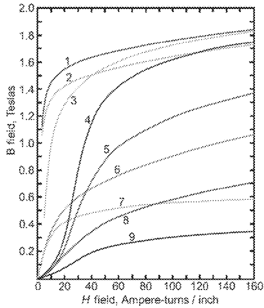
Magnetic flux density in different materials -- Sheet steel (1), Silicon steel (2), Cast steel (3), Tungsten steel (4), Magnel steel (5), Cast iron (6), Nickel (7), Cobalt (8), and Magnetite (9) -- as a function of the applied magnetic field.
